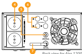
Back view for Aira 1200
