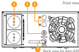
Back view for Aira 600
