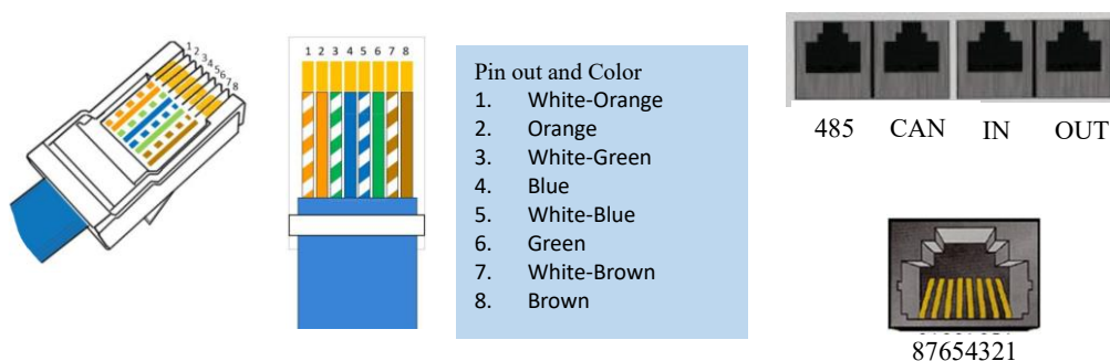
Figure 2-2 CAN,RS485,OUT,IN interface definition
